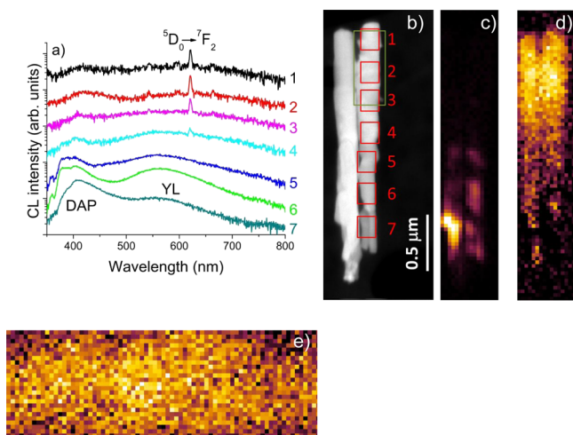
Figure 10. (a) Nano-CL spectra taken at seven points from the top (1) to the bottom (7) of a single NW implanted to a fluence of 1 \times 10^{14} at./cm 2 (20° incidence angle) and annealed at 1000 °C. The regions at which the spectra were taken are indicated with red rectangles in (b). (c,d) Luminescence intensity maps integrating the spectra in a wavelength region from 350 to 550 nm (c) and around the 622 nm Eu 3+ line (d). (e) Detail of the luminescence intensity map integrating the Eu 3+ emission peak at 622 nm in the region with highest Eu-emission marked with the bigger green rectangle in (b); the pixel size is 10 \times 10 nm 2 .
