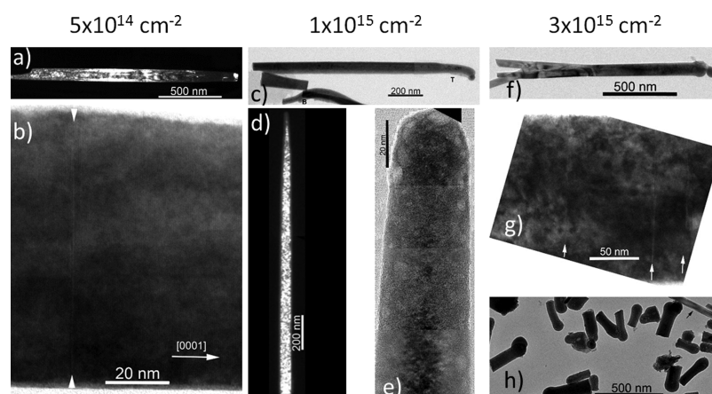
Figure 7. TEM images of as-implanted NWs implanted to a fluence of (a,b) 5 \times 10^{14} , (c–e) 1 \times 10^{15} , and (f–h) 3 \times 10^{15} \text{cm}^{-2} . Basal stacking faults are marked by white arrows.
