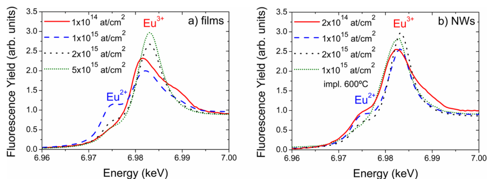
Figure 11. XANES spectra for selected thin films (a) and NWs (b) showing the coexistence of Eu in the 2+ and 3+ charge state and the possibility of decreasing the Eu 2+ fraction by HTHP annealing or implantation at elevated temperature plus RTA at 1000 °C. The Eu 2+ edge is found at a fixed position in all samples while the position of the Eu 3+ varies slightly for different implantation/annealing conditions.
