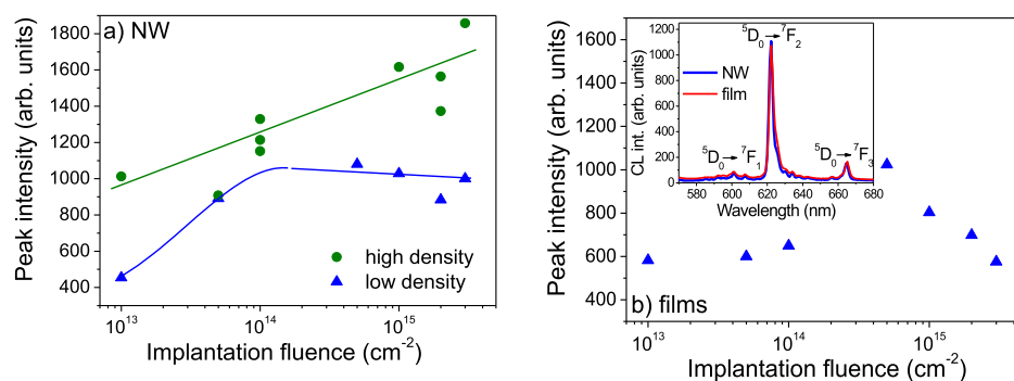
Figure 9. RT CL peak intensity of the Eu 3+ emission line at ~622 nm as a function of the fluence for NWs in regions with low and high NW density (a) and thin film reference samples (b). The inset in (b) compares typical CL spectra for NW and thin film samples.
