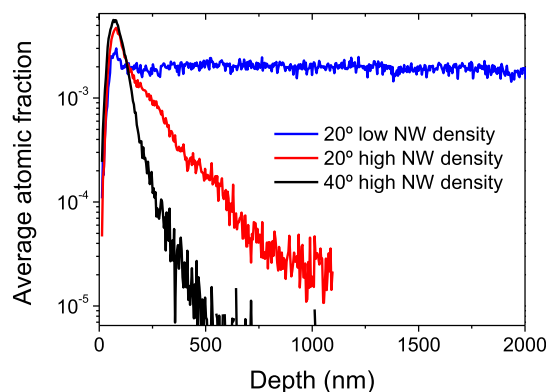
Figure 3. TRI3DYN simulation results showing the average atomic Eu fraction along the NW length for the three combinations of implantation angle, NW diameter, and density.
